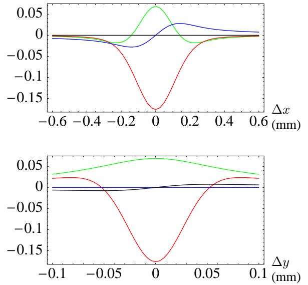
Figure 1: Perturbations due to the beam-beam effect during a luminosity scan in HERA's phase 2. In each figure the central curves describe the beam-beam displacements \delta x (blue) and \delta y (black) in mm. The lowest (red) and the highest (green) curves describe the relative change \delta\beta_y^e/\beta_y^e and \delta\beta_x^e/\beta_x^e of the beta functions respectively.
